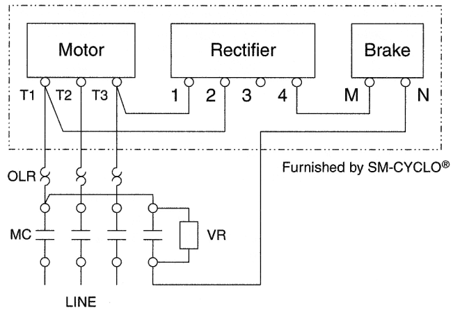
Fig. C-8b Fast Brake Action, High Voltage
