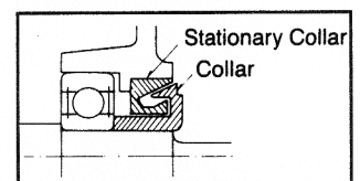
Fig. B-18 Slinger Type: Oil Lubed Units
