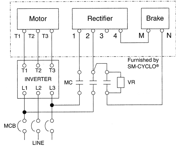
Fig. C-9b Fast Brake Action, High Voltage
