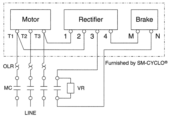
Fig. C-8d Fast Brake Action, Low Voltage
