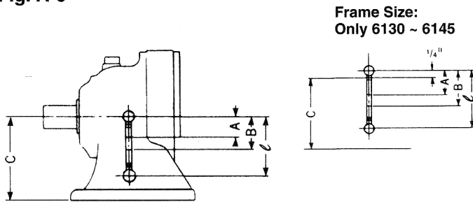
Foot Mount Horizontal Type Fig. A-6
