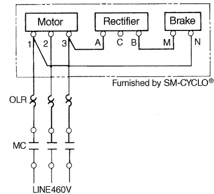
Fig. C-11b High Voltage 400 ~ 460V
