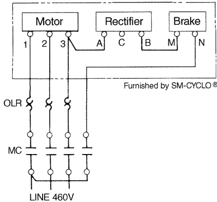
Fig. C-11d High Voltage 400 ~ 460
