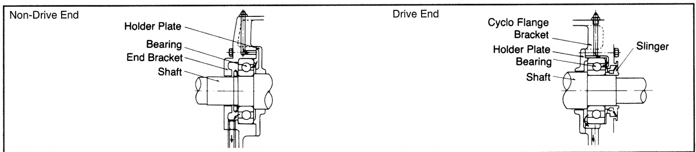
Fig. B-16 Typical Bearing Assembly
