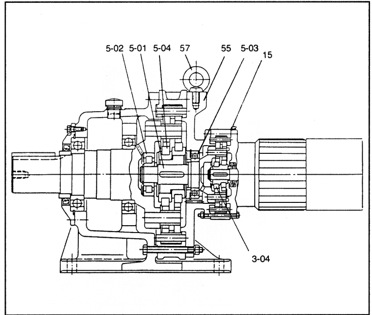
Fig. B-4 Gearmotor/Double Reduction
