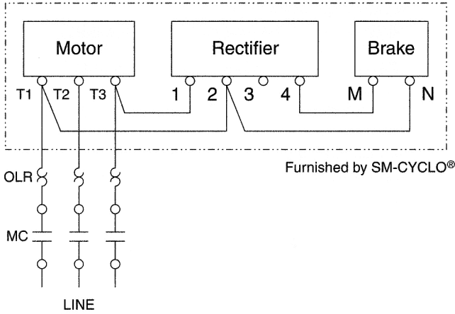
Fig. C-8a Normal Brake Action, High Voltage
