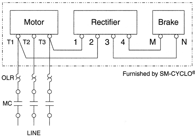
Fig. C-8c Normal Brake Action, Low Voltage
